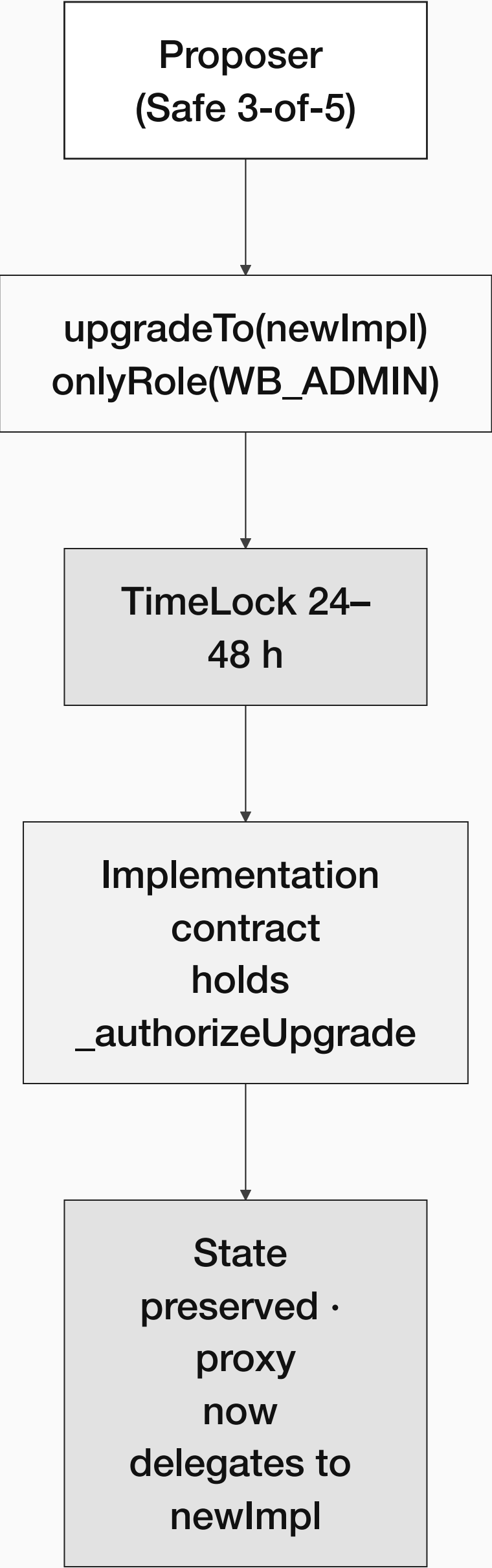
(a) UUPS upgrade path
